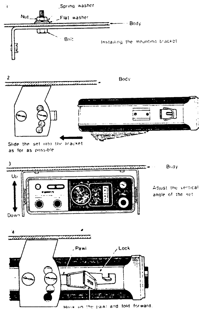
Fig. 6 Installing the Set on the Car
