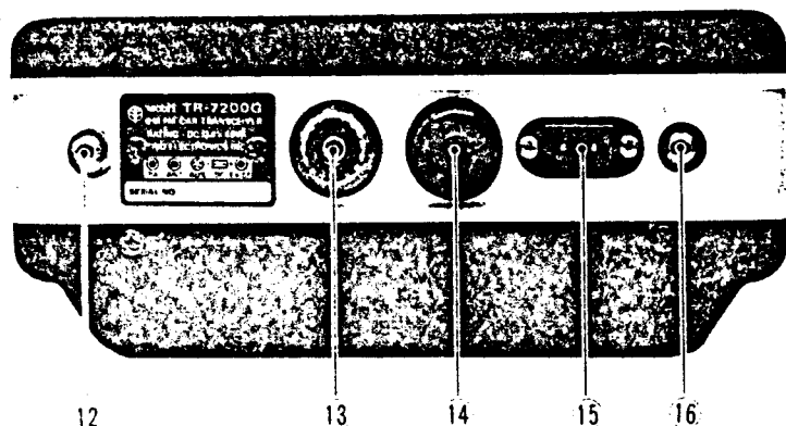
Fig. 2 Rear Panel
